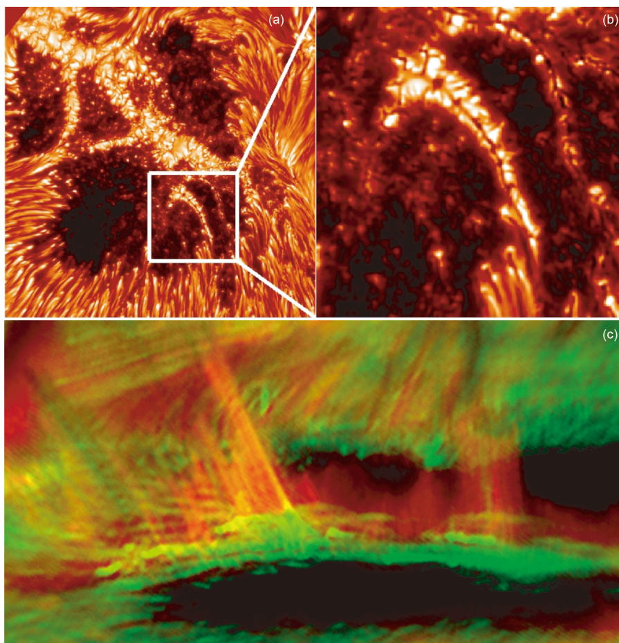
图1 (网络版彩色)GST观测到的黑子亮桥. (a) 太阳黑子及其本影中的亮桥; (b) 亮桥上的暗结 [49] ; (c) 亮桥上的倒Y型喷流 [50] Figure 1 (Color online) Observations of sunspot light bridges by Goode Solar Telescope (GST). (a) A sunspot with a light bridge (marked by a rectangle) spanning across the umbra; (b) dark knots on the light bridge in (a) [49] ; (c) inverted Y-shaped jets on a light bridge [50]
